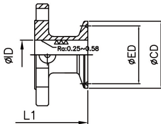
GKV-33T TRI-CLAMP FOR O.D TUBING
